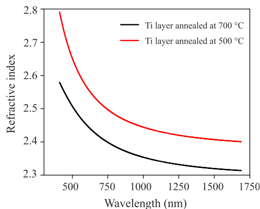
Fig. 2. Refractive index measurement of TiO 2 layer on ceramic substrate
